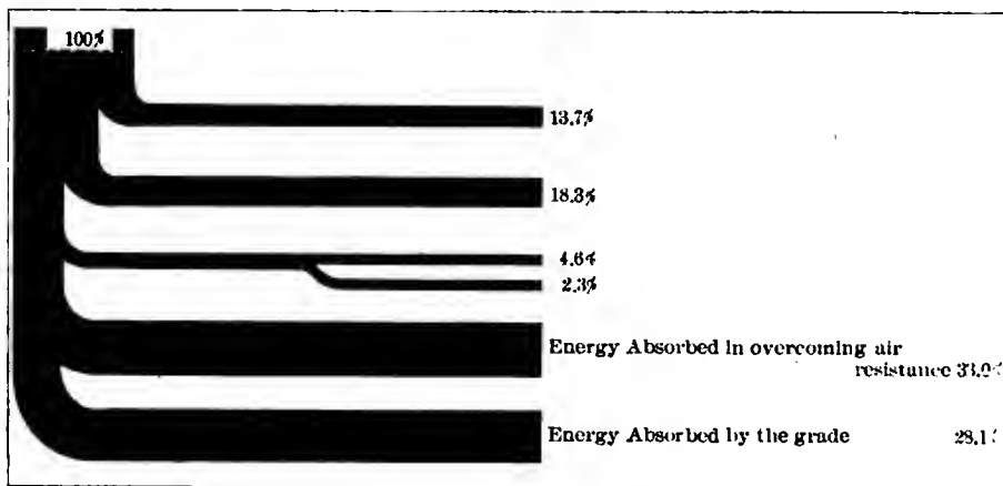
Fig. 3—Energy diagram of a 30-horsepower car running at 60 kilometers (37 miles) per hour, on a grade of 6 per cent. (relating to the energy available at the crankshaft); 33 per cent. of this energy is absorbed in wind resistance and 28 per cent. by the resistance of the grade
